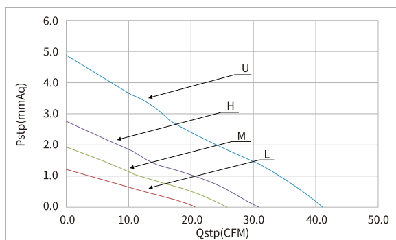
风扇P-Q曲线 / Fan performance curve
