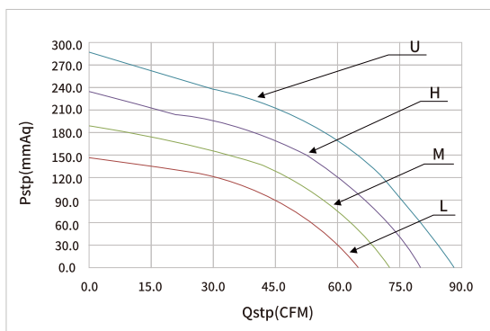
风扇P-Q曲线 / Fan performance curve
