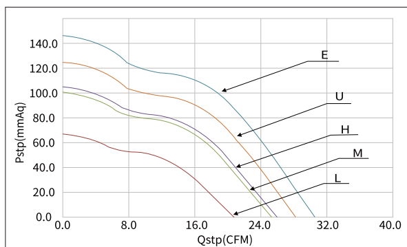
风扇P-Q曲线 / Fan performance curve
