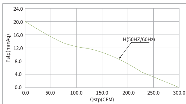
风扇P-Q曲线 / Fan performance curve
