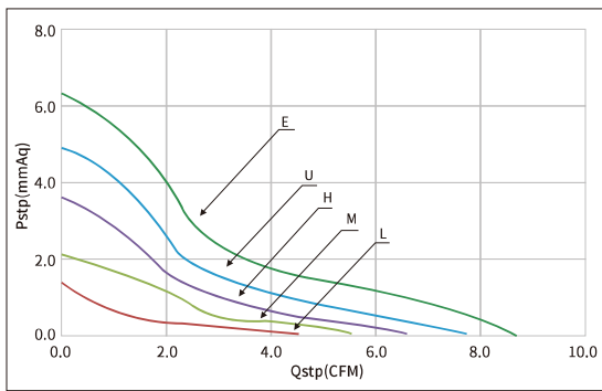
风扇P-Q曲线 / Fan performance curve
